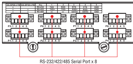
RS-232/422/485 Serial Port x 8
