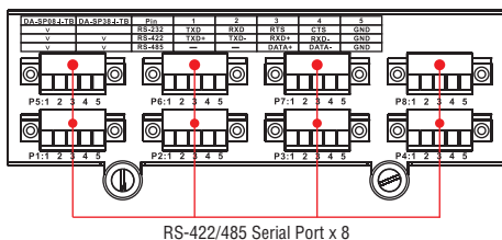
RS-422/485 Serial Port x 8
