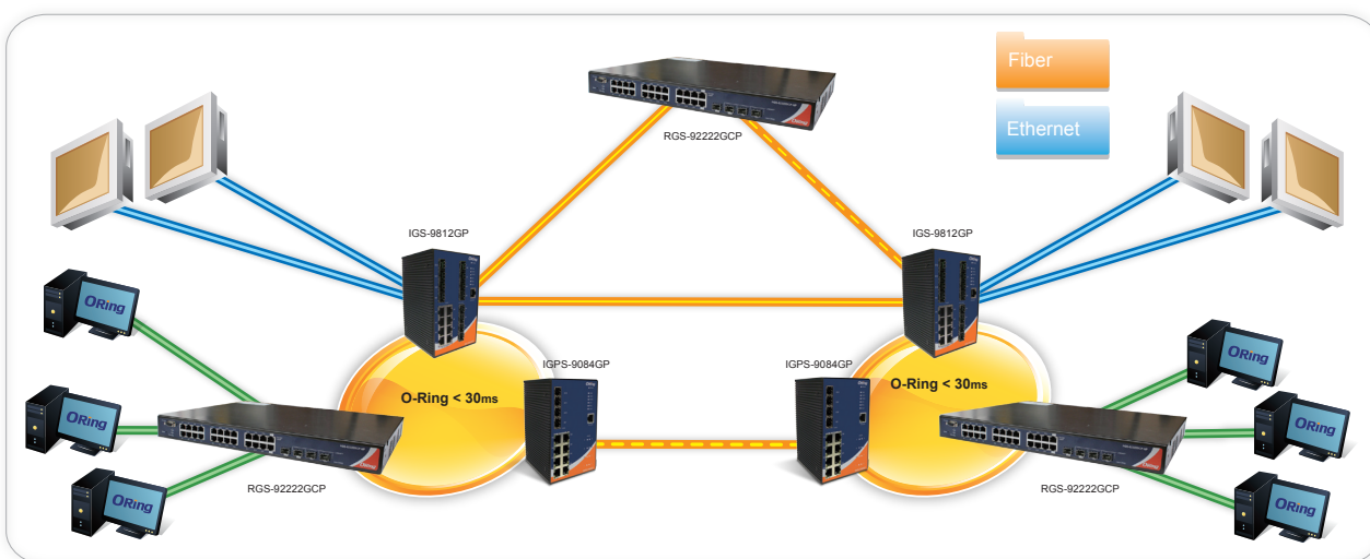
Network connection
