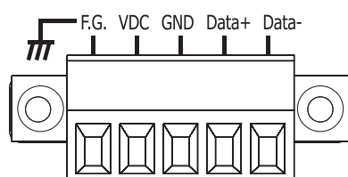
TPD-430 Rear View
