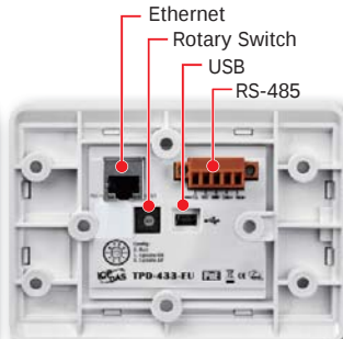
TPD-433-EU Rear View
