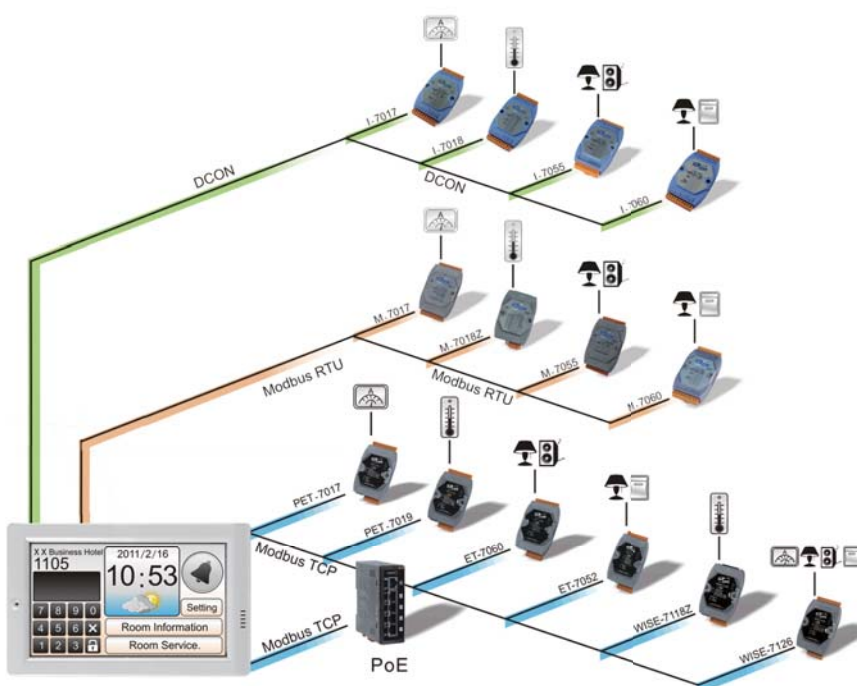
TPD-430/TPD-433 with US Outlet Box
