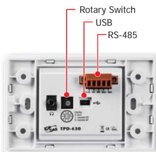
TPD-430 Rear View
