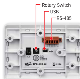
TPD-430-EU Rear View
