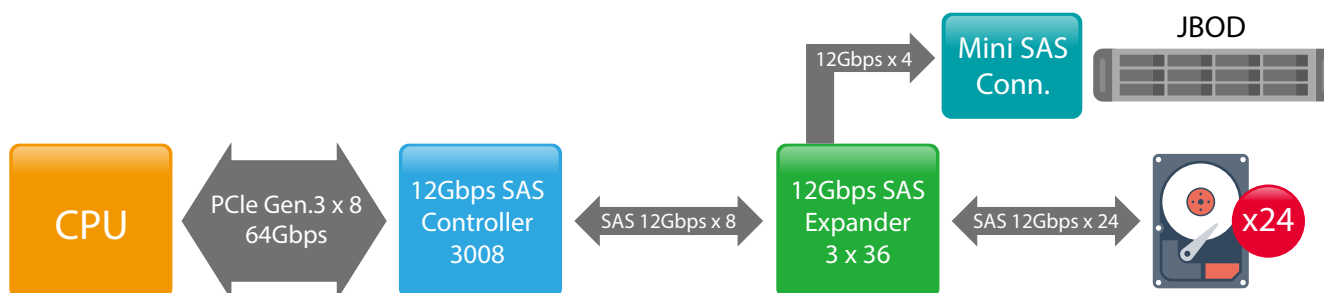
TVS-ECx80U-SAS R2 12Gb/s SAS model block diagram
