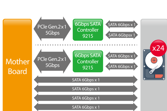
TS-x80U R2 SATA model block diagram
