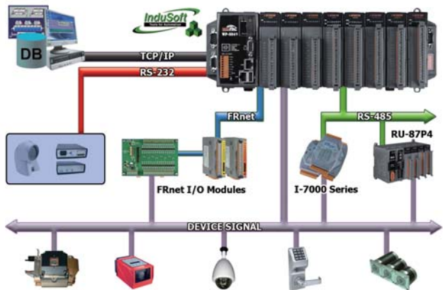
WP-8439 + I-87K I/O Modules
